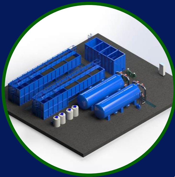
3D Drawings
